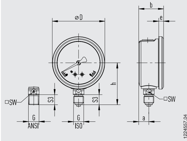
NS 50 [2"] and NS 63 [2 ½"], lower mount (radial)
